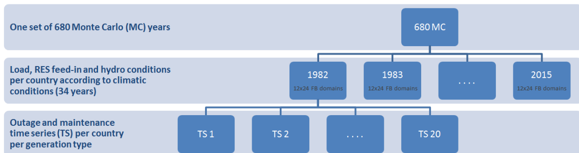
Figure 16 Rationale behind the construction of simulated years, based on 34 climate years and 20 scenarios for thermal availability
